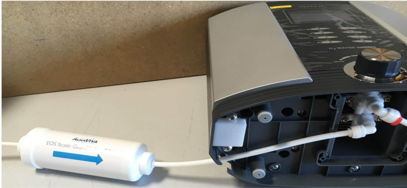
Filter arrow must face ionizer as shown in photo.
